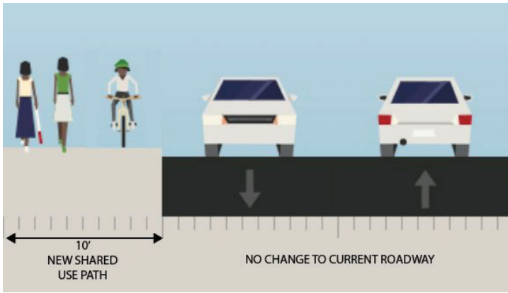
10' Shared Use Path
