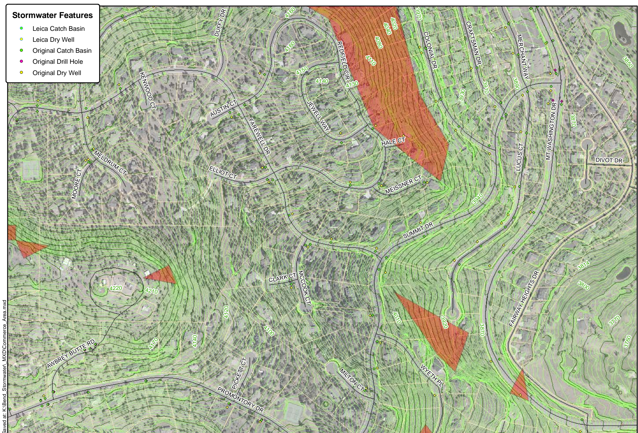
Figure 5 Fairway Heights City of Bend Stormwater Master Plan Map Date: May 31, 2007
